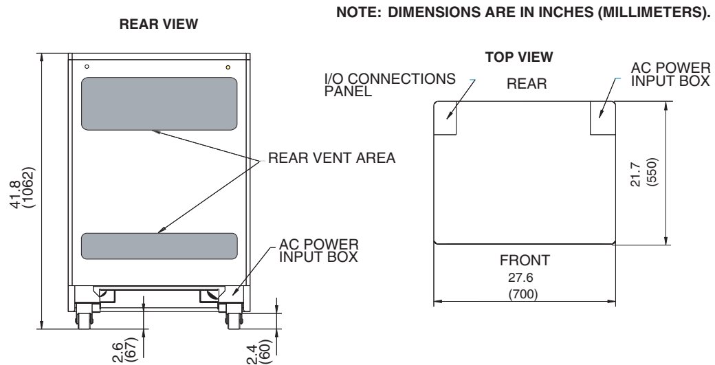
Figure 4-8 Power Distribution Unit (NGPDU)
