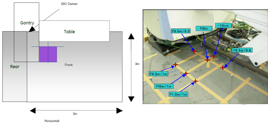
Figure 4-15 Fluoro Stand Position
