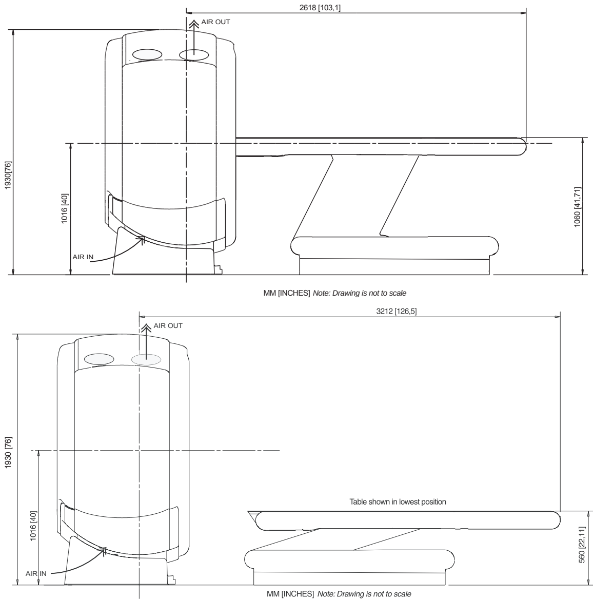
Figure 4-6 Table and Gantry (Side View)
