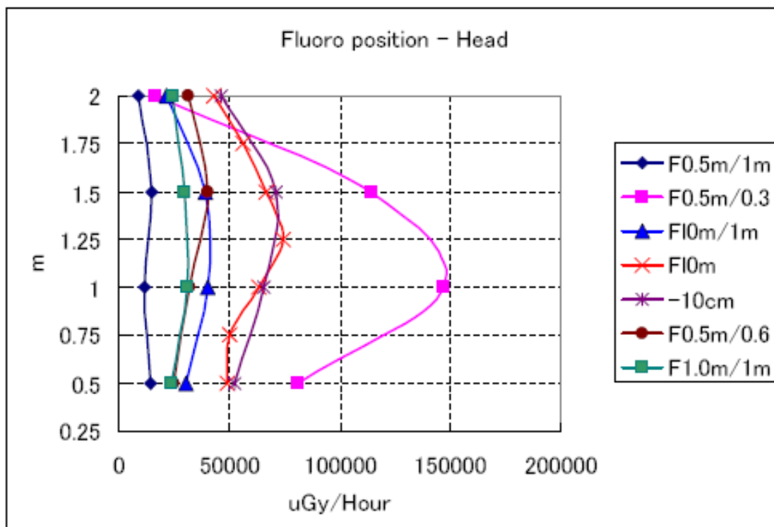
Figure 4-17 Scatter Plot of Fluoro - Head
