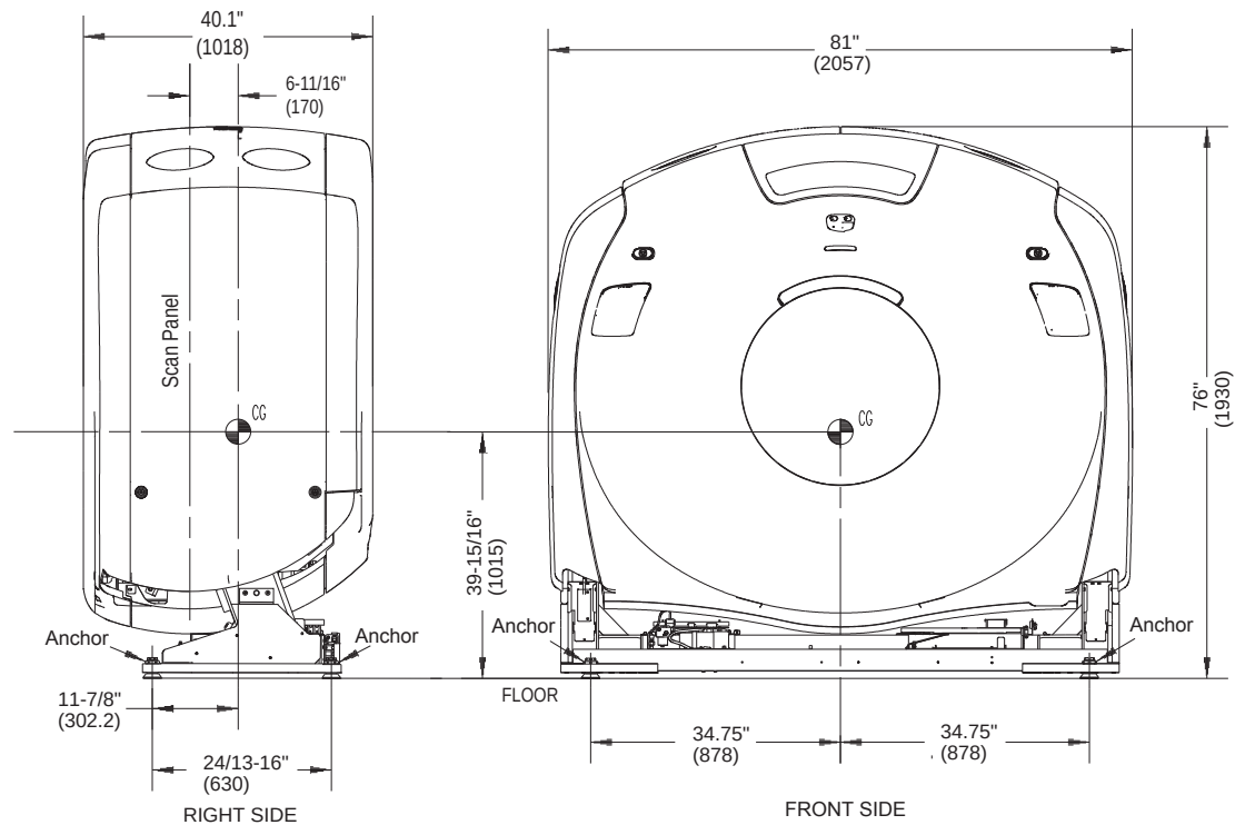
Figure 6-2 Gantry (CT2)
