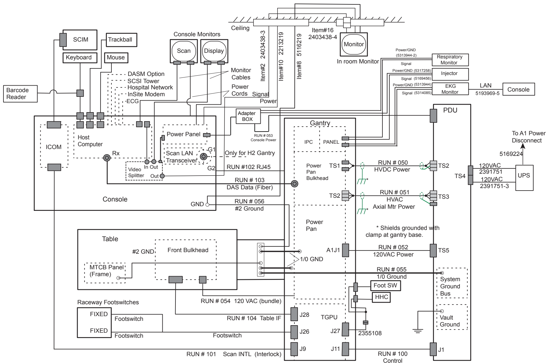
Figure 9-2 System Interconnect Diagram (With IPC Board)
