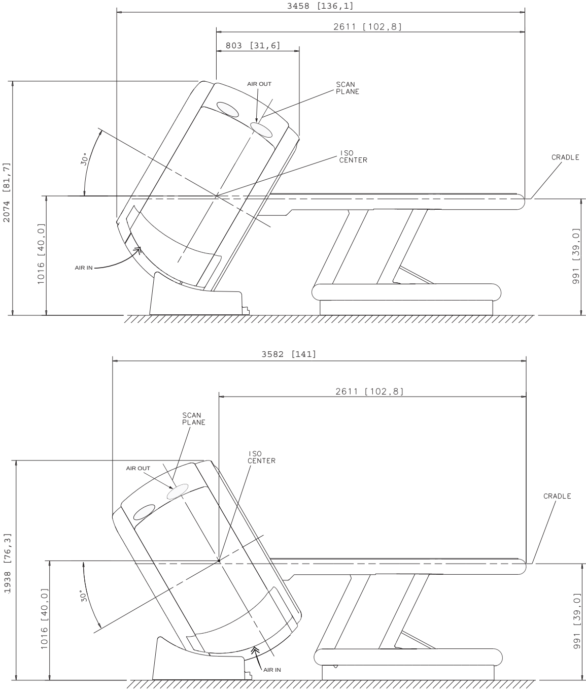
Figure 4-7 Gantry shown tilted +30° (top) and -30° (bottom)
