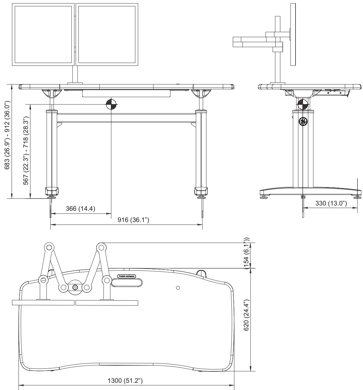
Figure 4-11 Freedom Workspace Table (part 5168666)
