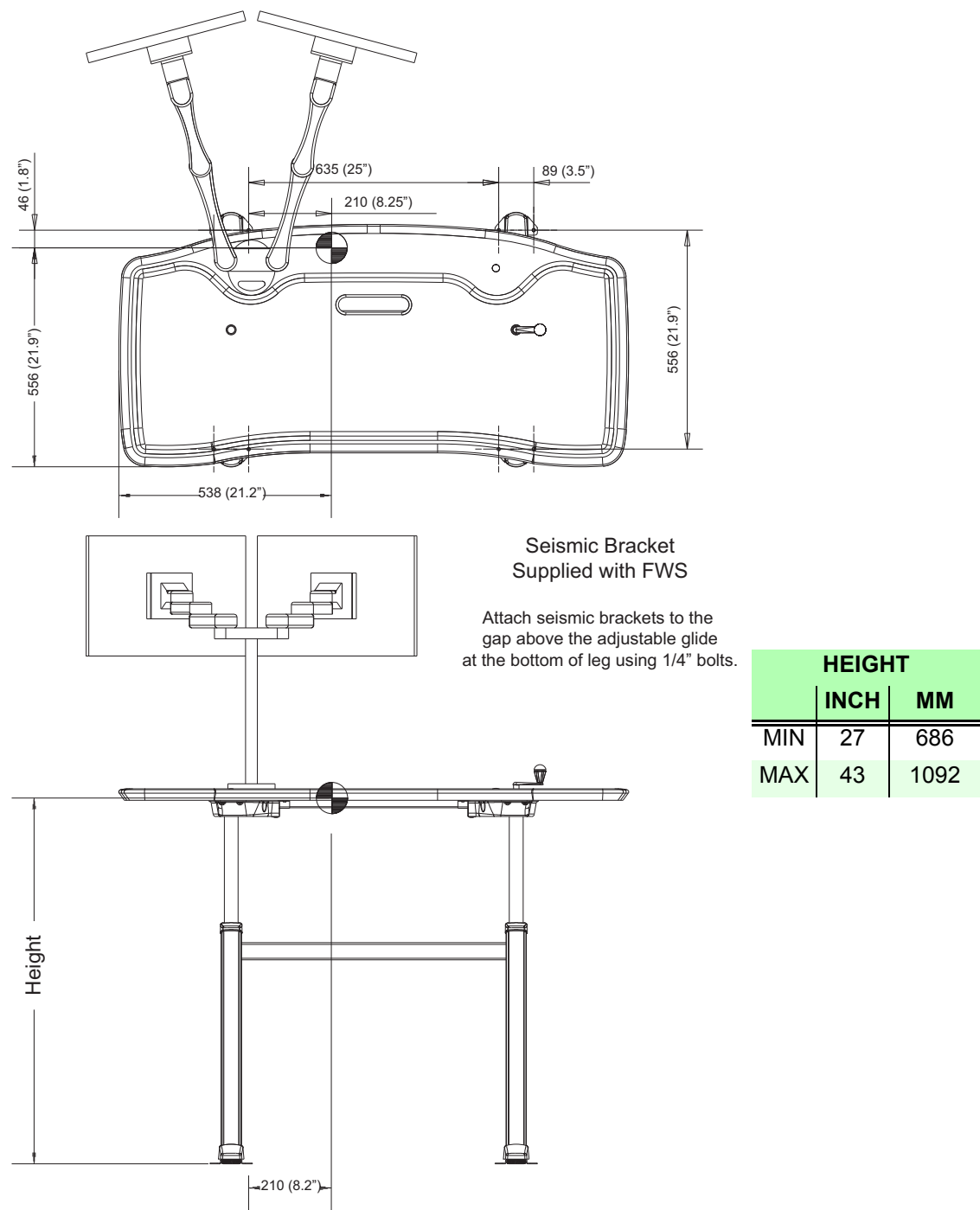
Figure 4-10 Freedom Workspace Table (part 5160735)
