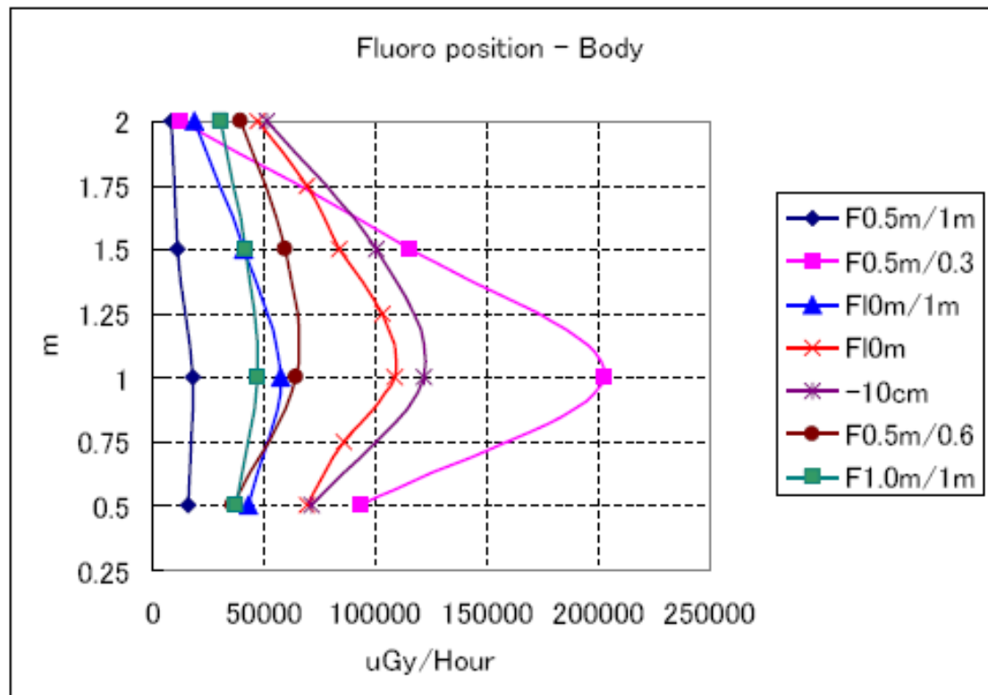
Figure 4-16 Scatter Plot of Fluoro - Body
