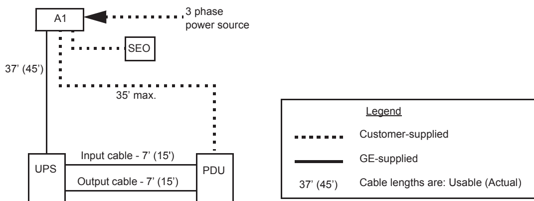
Figure 9-4 Typical UPS Interconnect
