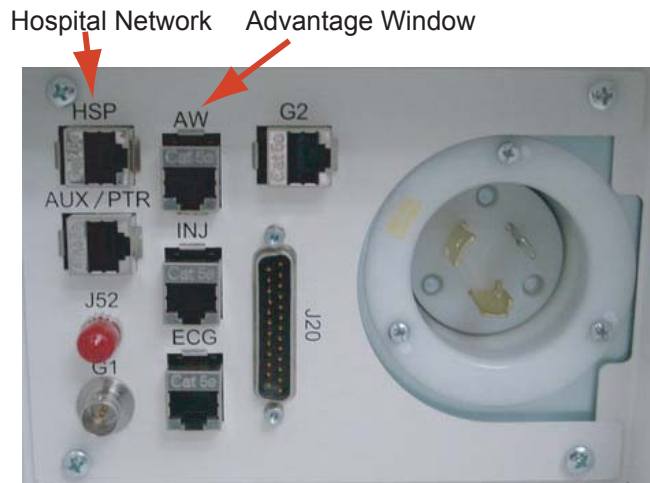
Figure 4-12 Console Rear Bulkhead
