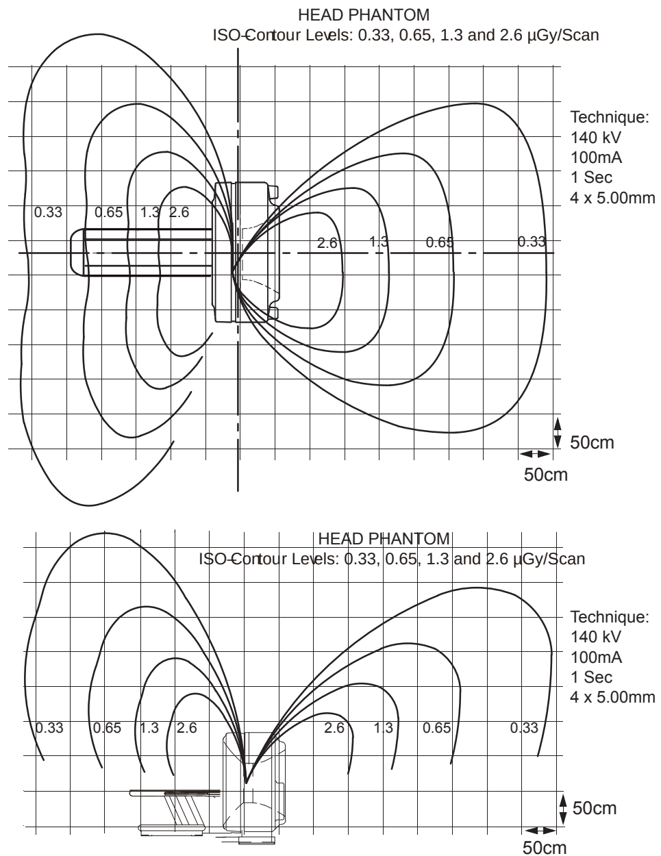
Figure 4-13 Typical Scatter Survey (Head Filter)
