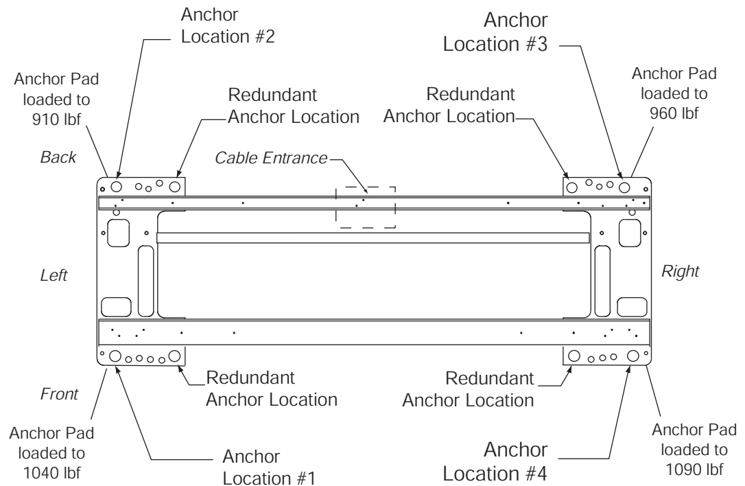
Figure 6-2 Gantry (CT2)
