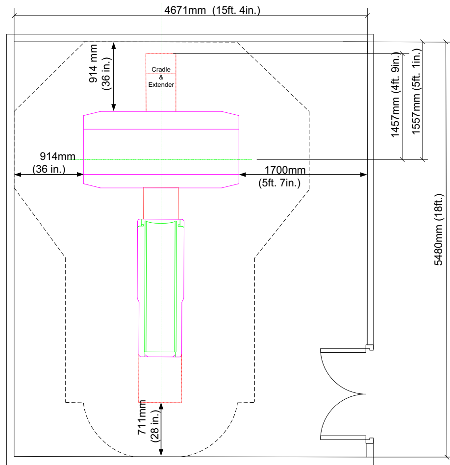
Figure 4-4 Minimum Room layout for Short Footprint function
