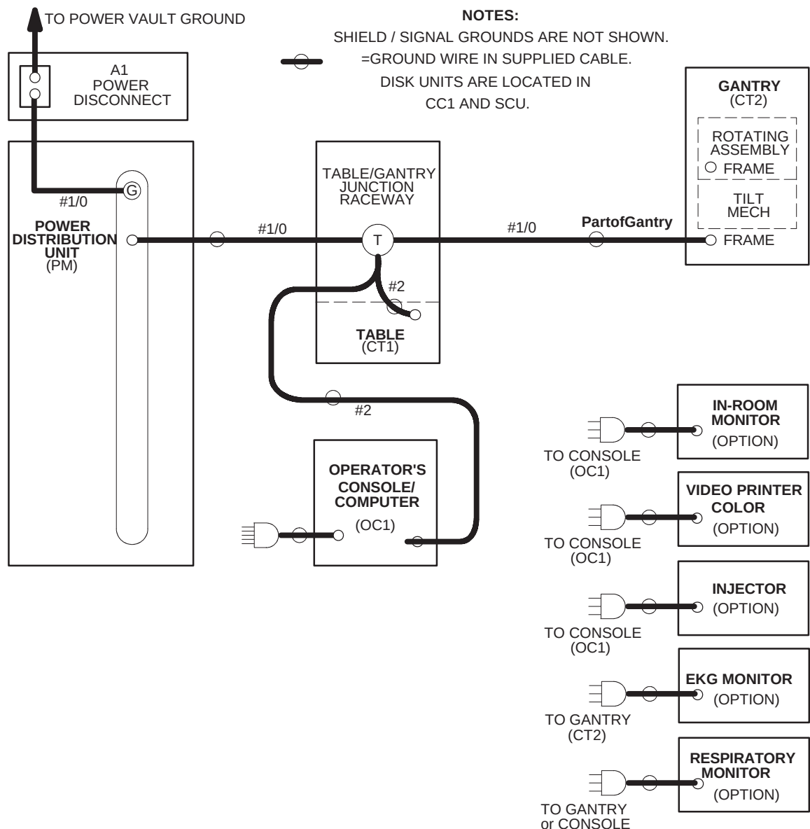
Figure 8-1 System Ground Map
